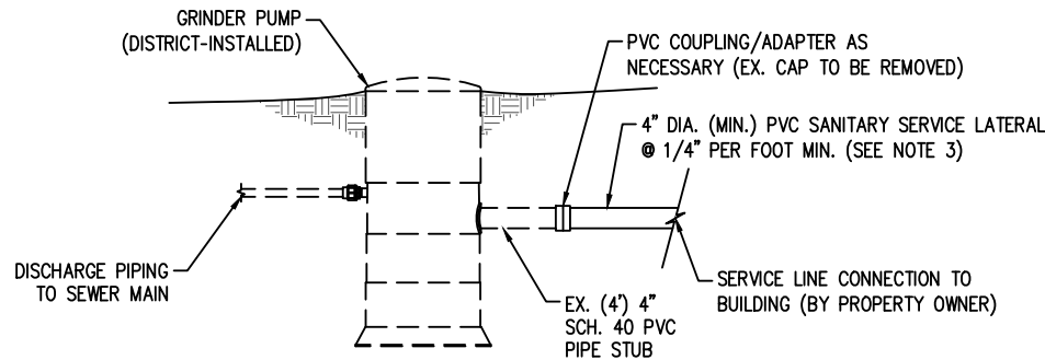
TYPICAL GRINDER PUMP CONNECTION
