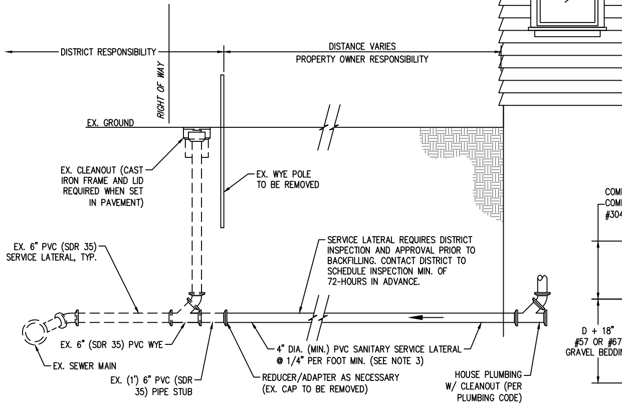
TYPICAL GRAVITY SEWER CONNECTION
