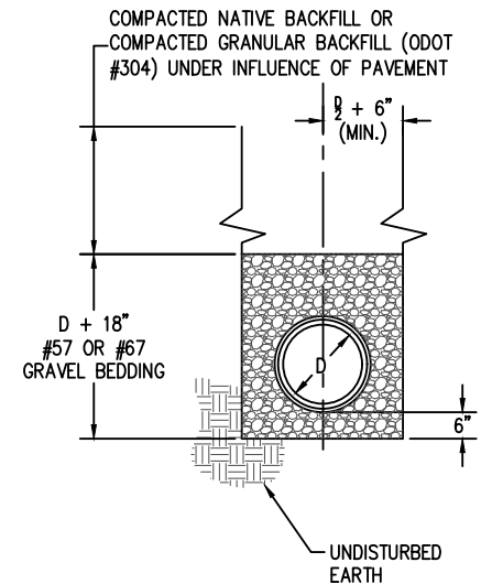
TYPICAL TRENCH
